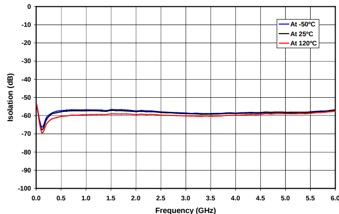
Figure 2. Isolation vs. Frequency per Temperature
