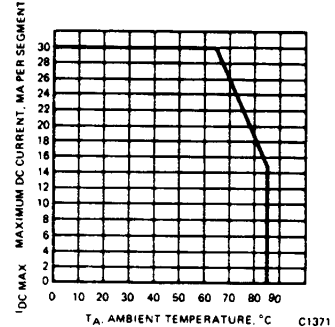
Fig. 5. Maximum DC Current vs. Temperature
