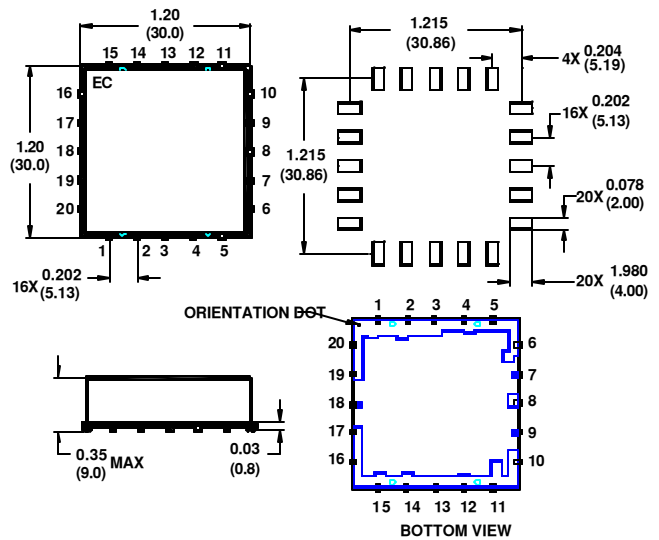
SM-85 Case Style
