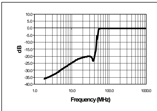
Low Pass Filter Output Return Loss
