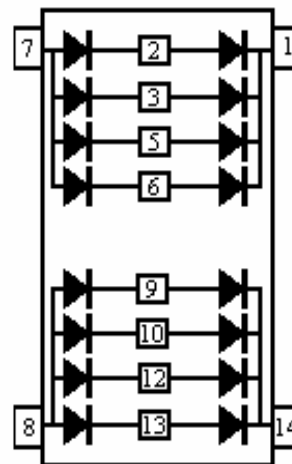
CIRCUIT CONFIGURATION
