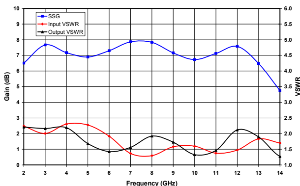
Figure 3. Small Signal Gain and Input and Output VSWR at V_D=8V .
