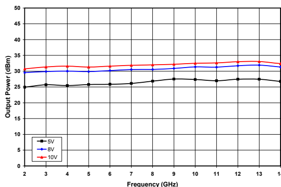
Figure 2. Saturated Output Power vs. Frequency and Drain Voltage at 25% IDSS.
