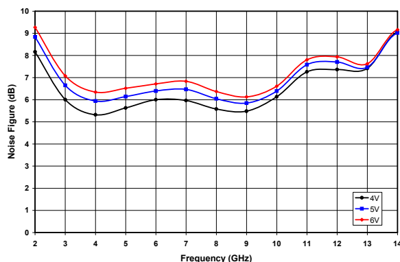
Figure 5. Noise Figure vs. Frequency and Drain Voltage.
