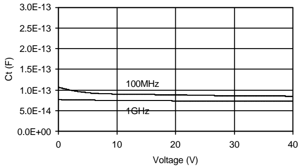
Ct vs Voltage (@ 100MHz & 1GHz) MA4SPS421
