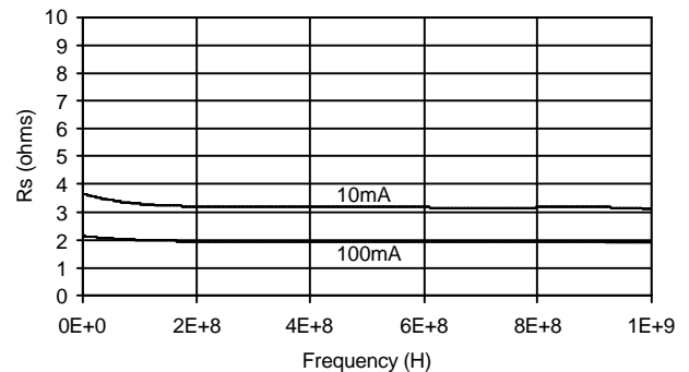
Rs vs Frequency (@ 10mA & 100mA) MA4SPS422
