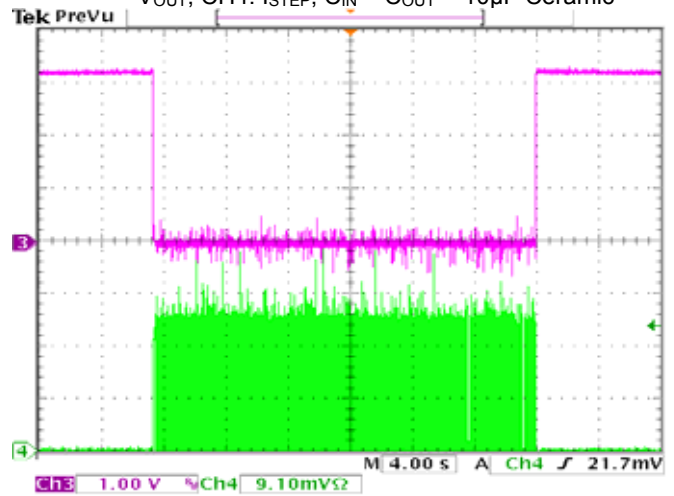
SHORT CIRCUIT AND RECOVERY V_{OUT} , CH4: I_{STEP} , C_{IN} = C_{OUT} = 10\mu\text{F} Ceramic
