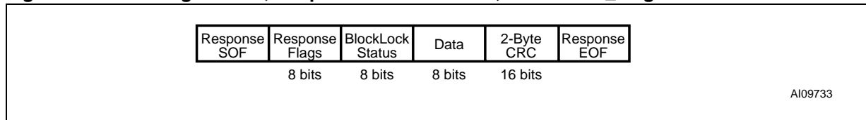
Figure 28. Read Single Block, Response Frame Format, when Error_Flag is not Set
