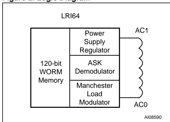
Figure 2. Logic Diagram
