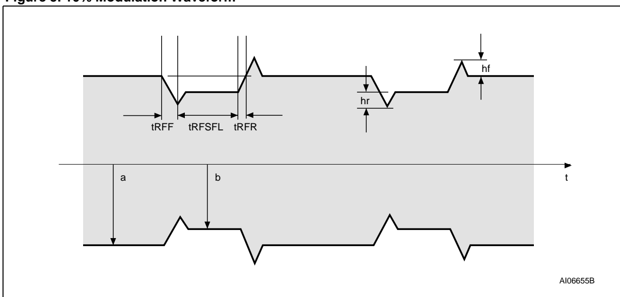
Figure 5. 10% Modulation Waveform
