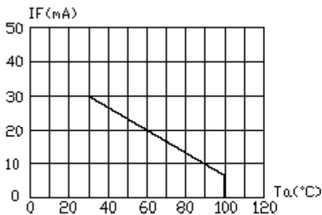
FIG.5 MAXIMUM FORWARD CURRENT VS. AMBIENT TEMPERATURE ( T_{jmax}=120^{\circ}C )
