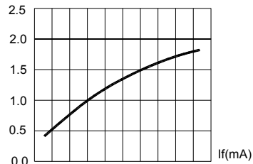
FIG.3 RELATIVE LUMINOUS FLUX VS. FORWARD CURRENT
