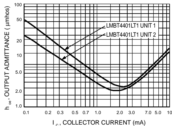
Figure 14. Output Admittance
