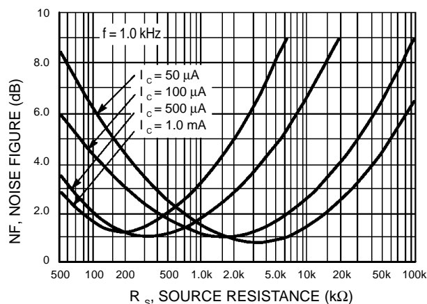
Figure 10. Source Resistance Effects
