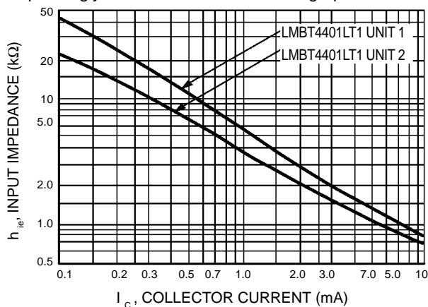
Figure 12. Input Impedance
