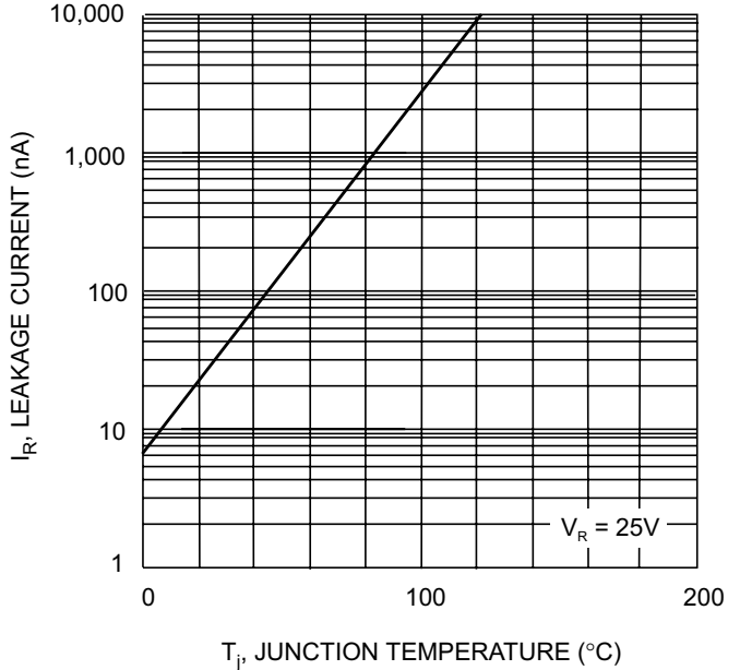
Fig. 4 Leakage Current vs. Junction Temperature
