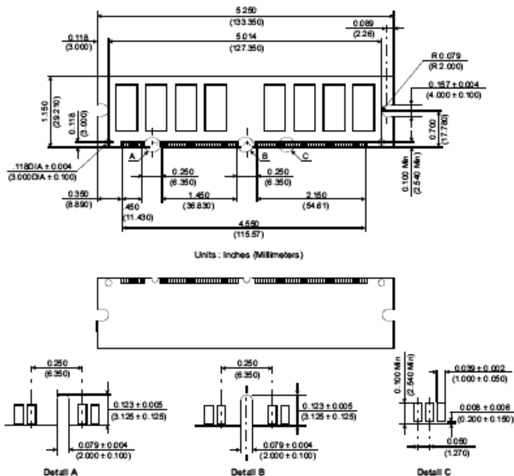
Figure 1: KVR133X64C3/256 168-Pin SDRAM Module
