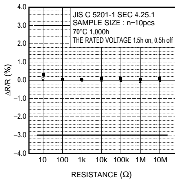
Fig.14 Endurance (at70°C)
