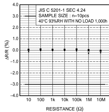
Fig.13 Damp heat , Steady state
