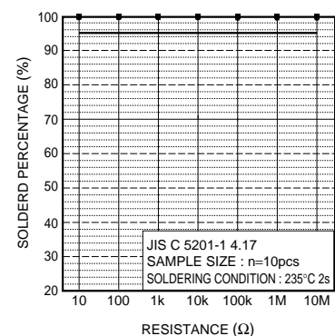
Fig.10 Solderability
