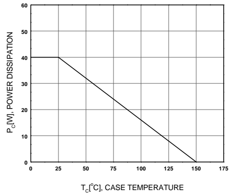
Figure 8. Power Derating
