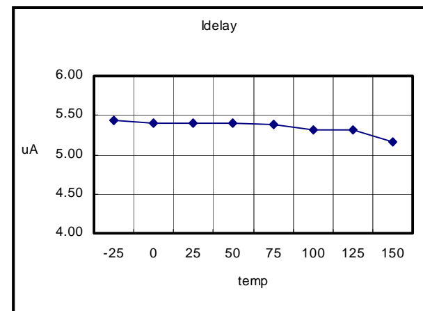
Figure 6. Shutdown Delay Current
