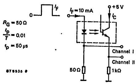
Fig. 2 Test circuit, saturated operation
