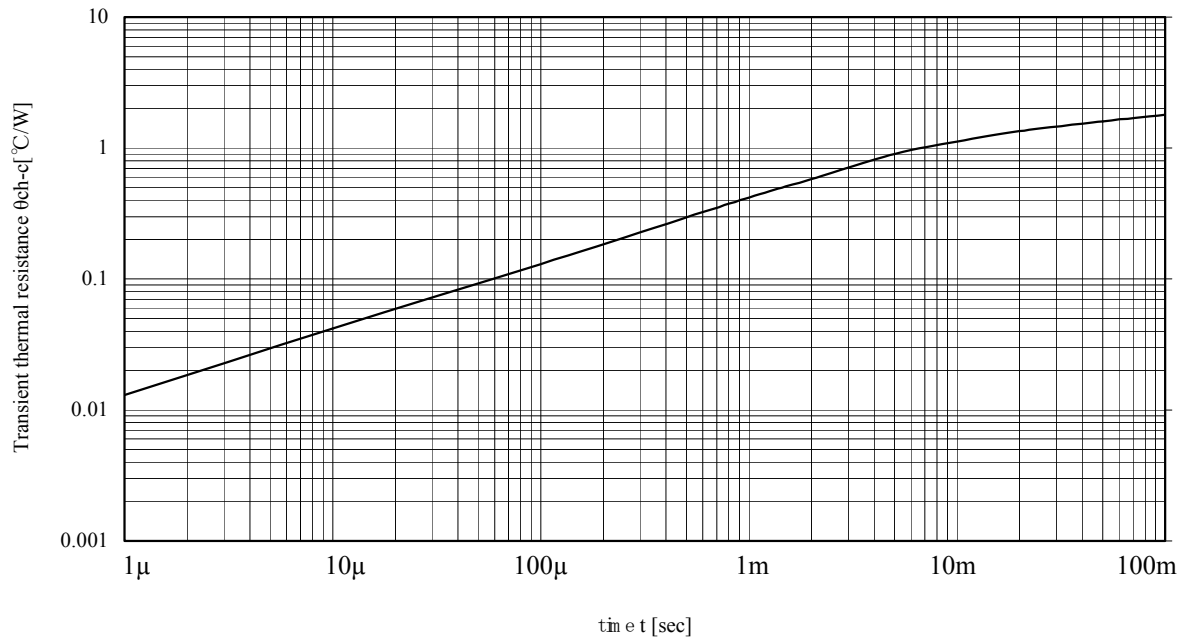
IRIS-G6651 Transient thermal resistance curve
