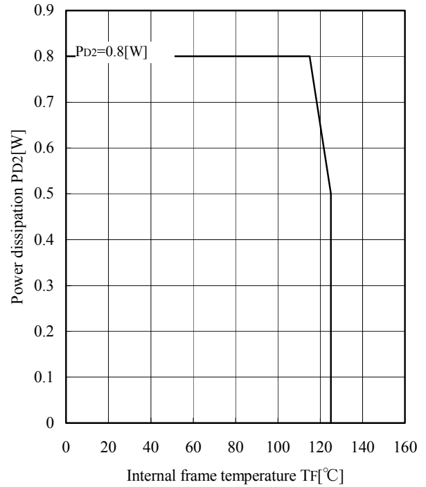
IRIS-G6651 MIC TF-PD2 Curve
