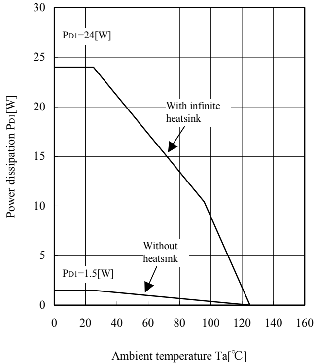
IRIS-G6651 MOSFET Ta-PD1 Curve
