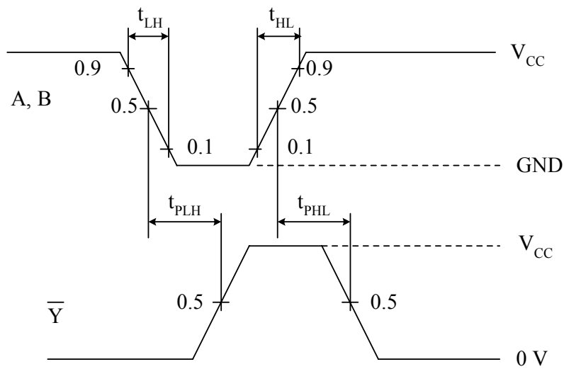
- Time diagram of input and output pulses
