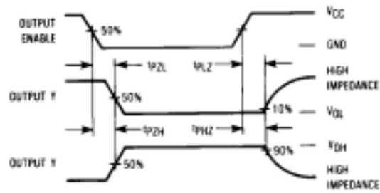
Figure 3. Switching Waveforms
