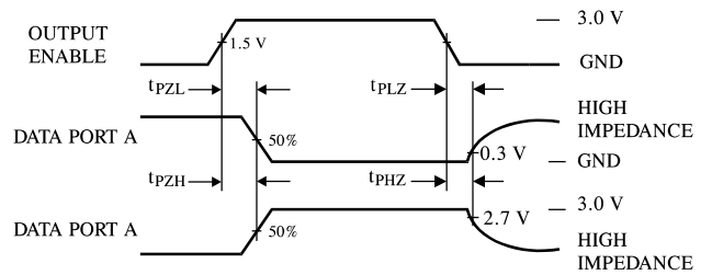
Figure 5. Switching Waveforms
