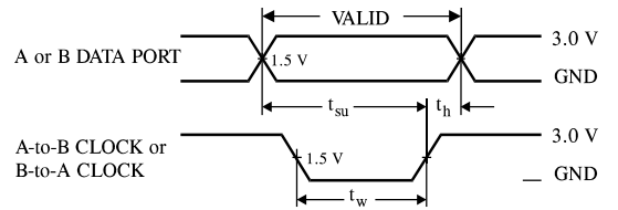
Figure 7. Switching Waveforms
