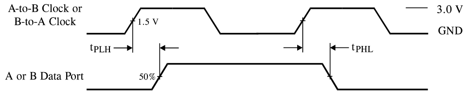
Figure 1. Switching Waveforms
