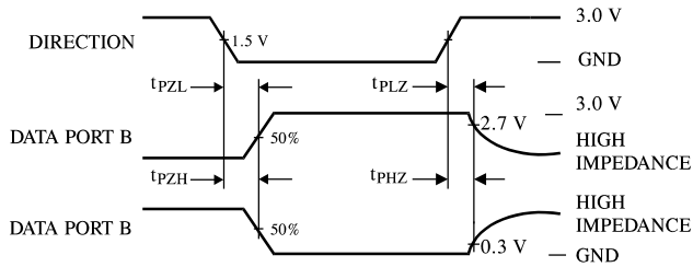
Figure 6. Switching Waveforms
