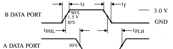
Figure 3. A Data Port = Output, B Data Port = Input
