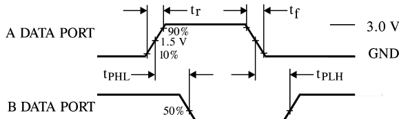
Figure 2. A Data Port = Input, B Data Port = Output
