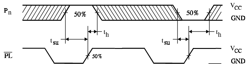
Figure 7. Switching Waveforms
