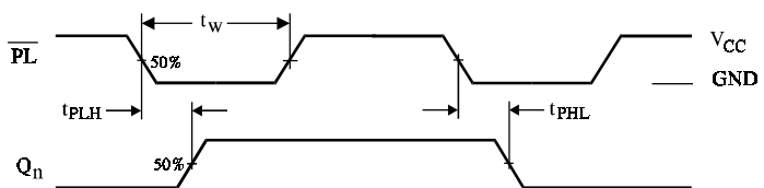
Figure 4. Switching Waveforms
