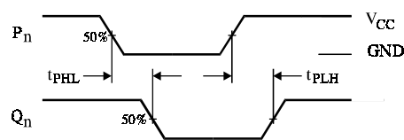
Figure 3. Switching Waveforms
