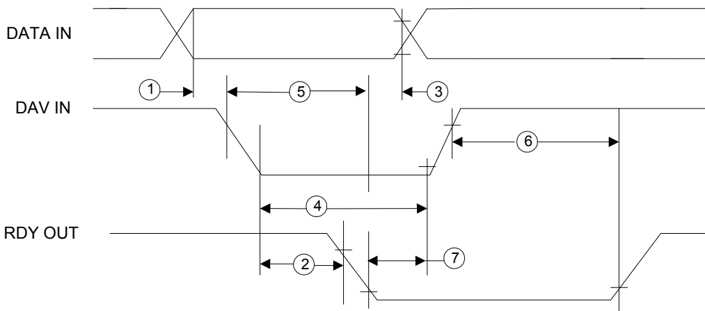
Figure 68. Fully Interlocked Mode (Input Handshake)
