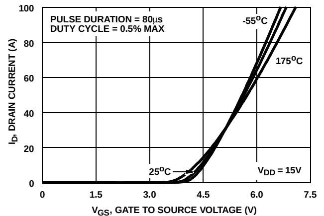
FIGURE 8. TRANSFER CHARACTERISTICS
