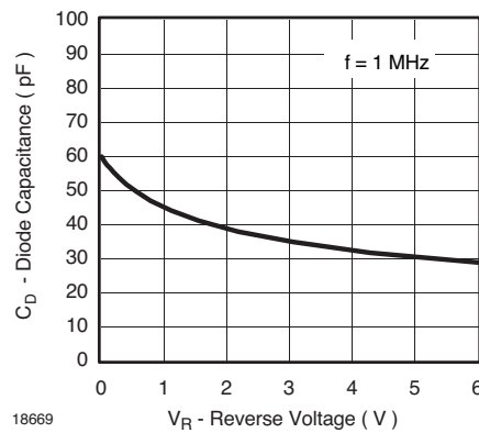
Figure 4. Typical Capacitance vs. Reverse Voltage
