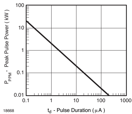
Figure 3. Non-Repetitive Peak Pulse Power vs. Pulse Time
