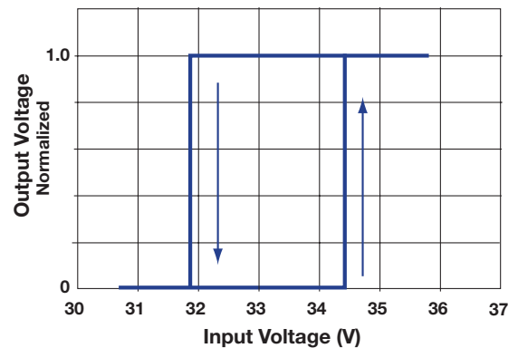
Undervoltage Hysteresis
