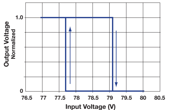
Overvoltage Hysteresis
