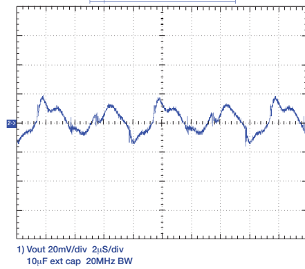
Voltage Ripple
