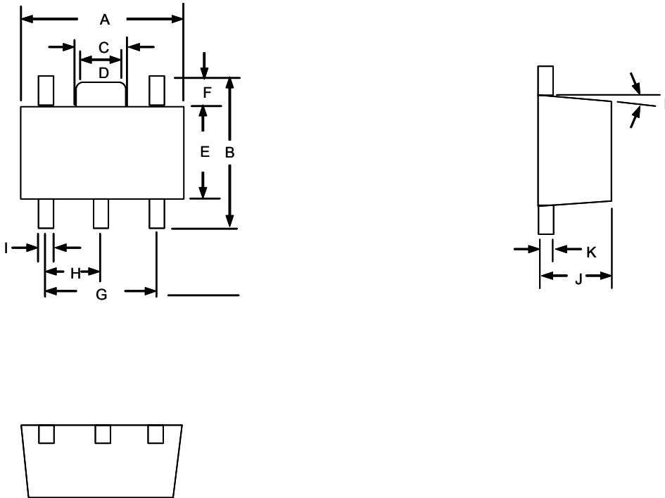
SOT-89-5 Package
