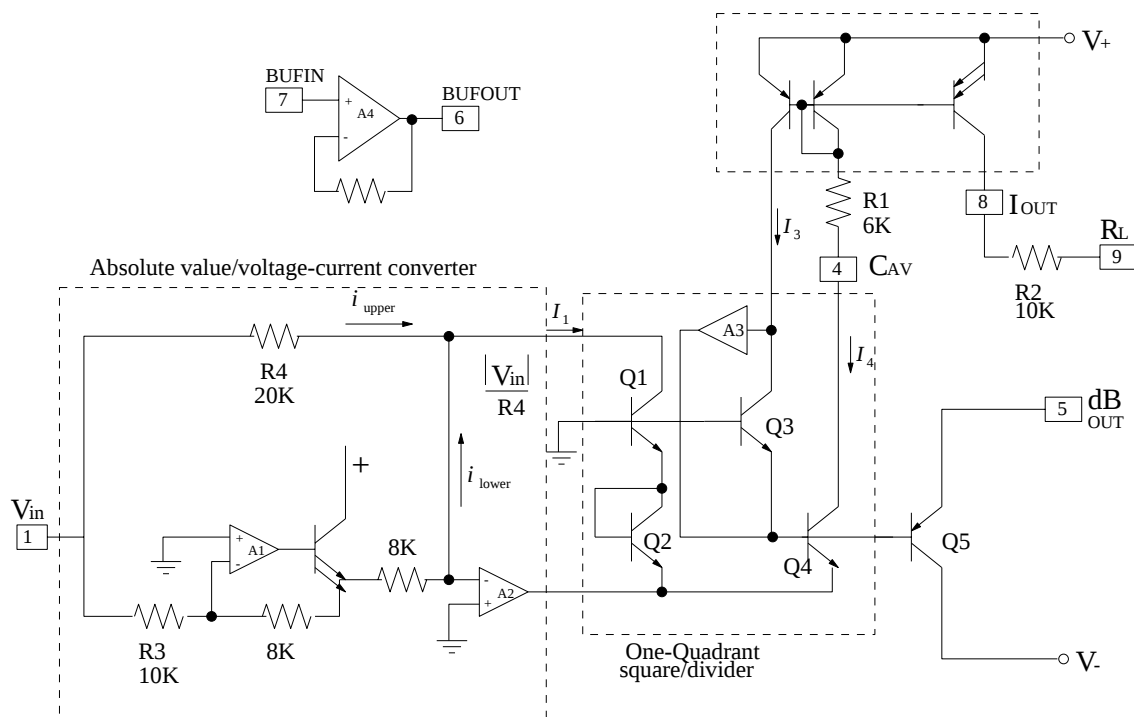
Figure 1. ES636 Simplified Schematic
