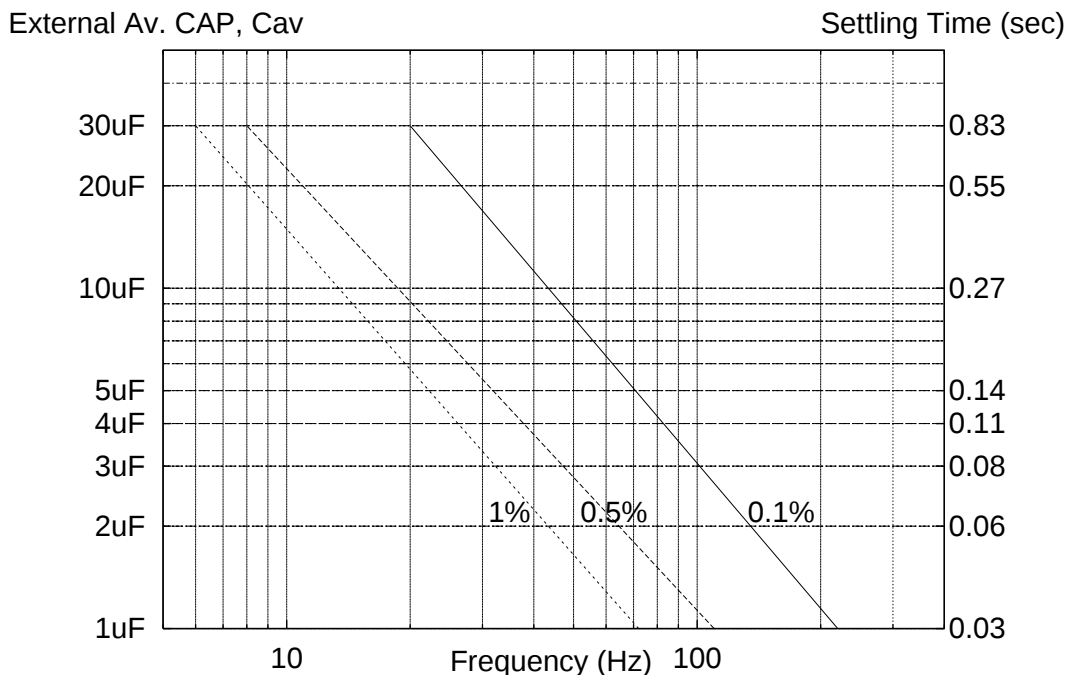
Figure 4. Errors/Settling Time Graph for Standard Connection
