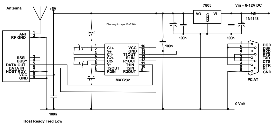
Figure 3 Application Circuit
