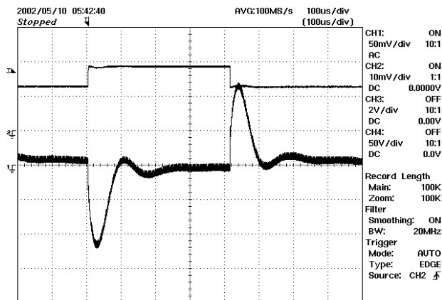
Figure 28 – Output Transient Response. 50% to 75% to 50% Load Step, 72 VDC Input. Upper Trace: Output Current, 2 A/div. Bottom Trace: Output Voltage, 50 mV/div, 100 \mu s/div.
