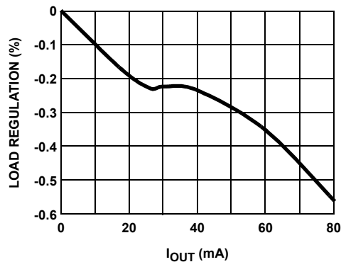
FIGURE 11. V_{ON} LOAD REGULATION
