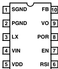
EL7532 (10 LD MSOP) TOP VIEW
