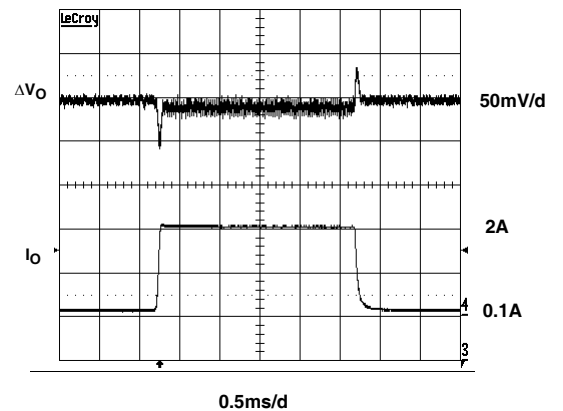
FIGURE 12. TRANSIENT RESPONSE
