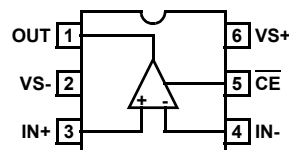
EL5164 (6-PIN SOT-23) TOP VIEW
