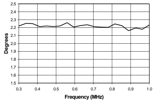
Phase Unbalance
