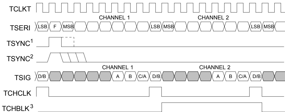
Figure 12-17. Transmit-Side Boundary Timing (with Elastic Store Disabled)
