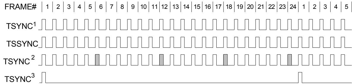
Figure 12-16. Transmit-Side ESF Timing
