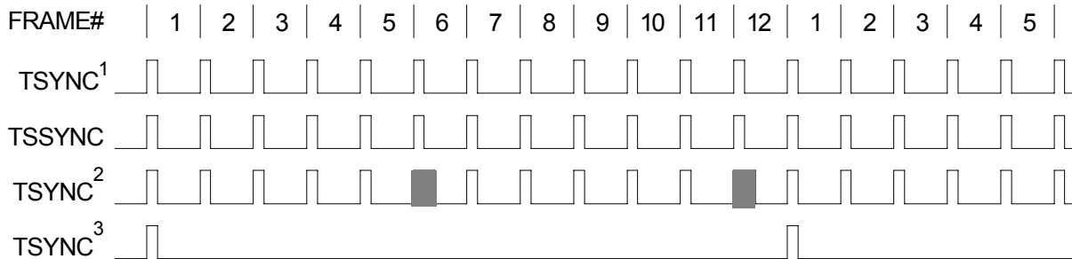
Figure 12-15. Transmit-Side D4 Timing
