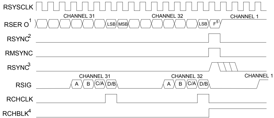
Figure 12-14. Receive-Side 2.048MHz Boundary Timing (Elastic Store Enabled)
