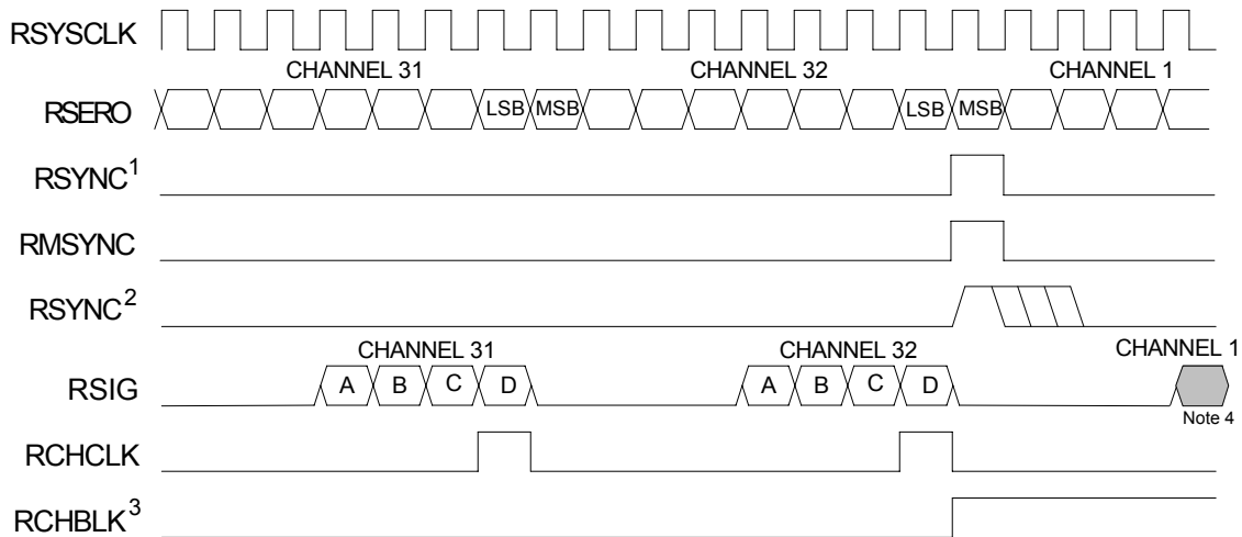
Figure 12-23. Receive-Side Boundary Timing, RSYCLK = 2.048MHz (E-Store Enabled)
