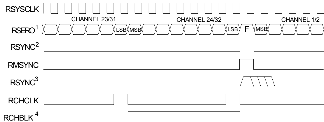
Figure 12-22. Receive-Side Boundary Timing, RSYCLK = 1.544MHz (E-Store Enabled)
