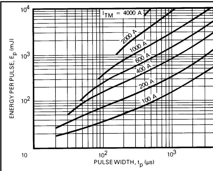
Fig.10 Energy per pulse for trapezoidal pulses
