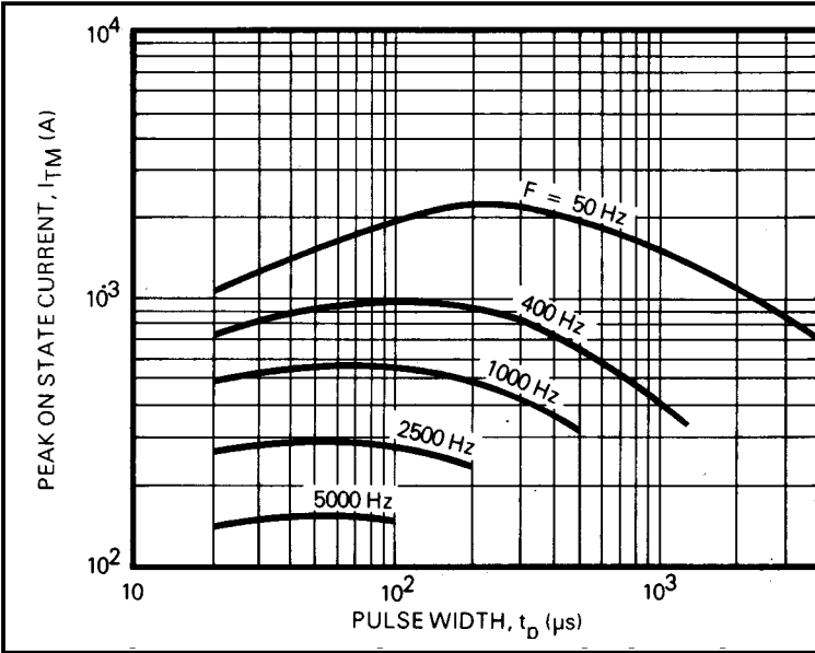
Fig.9 Maximum allowable peak on-state current vs pulse width for T_{case} = 90^\circ C
