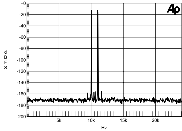
Figure 21b. IMD, 10 kHz and 11 kHz -7 dBFS, 96 kHz:48 kHz
