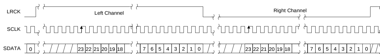
Figure 17. Right-Justified, 24-Bit Data
