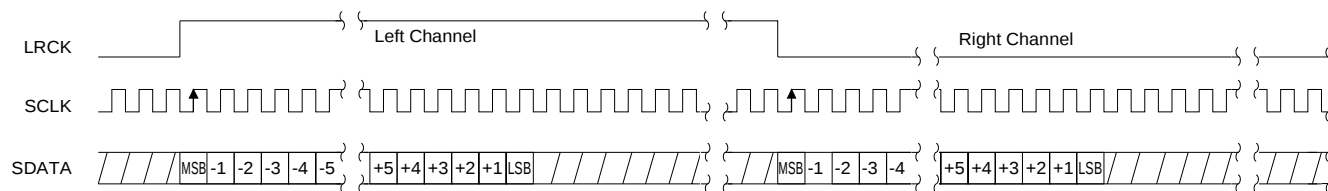
Figure 16. Left-Justified, up to 24-Bit Data
