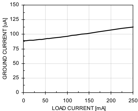
Ground Current vs. Load Current ( V_{IN}=3.3V )
