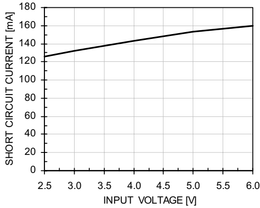
Short Circuit Current vs. Input Voltage
