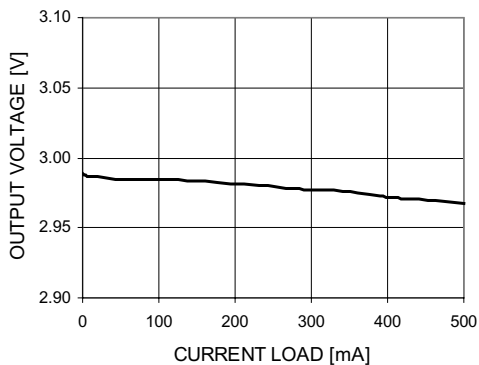
Figure 1. Load Regulation
