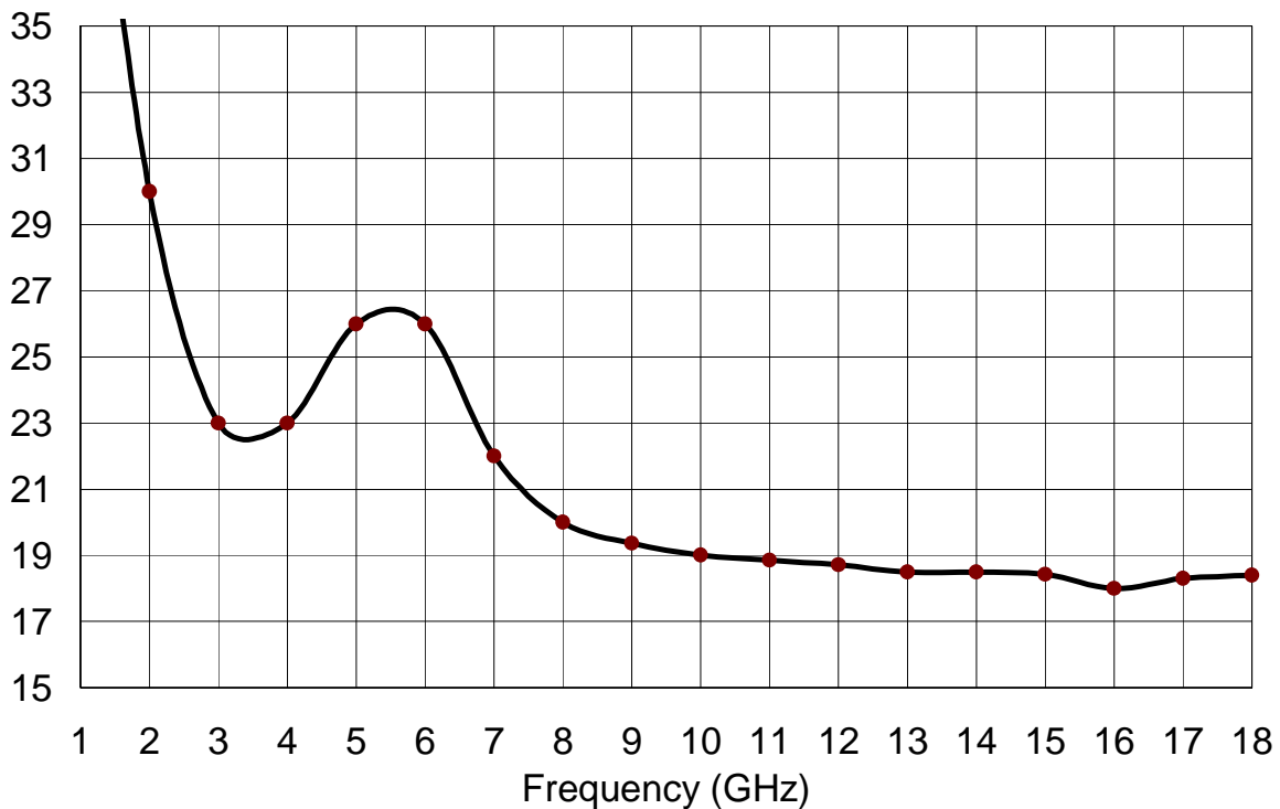
Isolation between channels versus frequency (dB)
