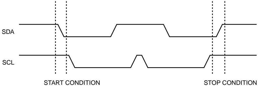
Figure 3. Start/Stop Condition
