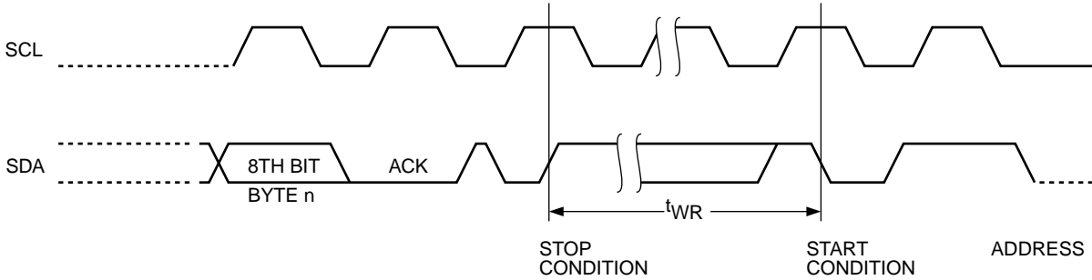
Figure 3. Start/Stop Condition
