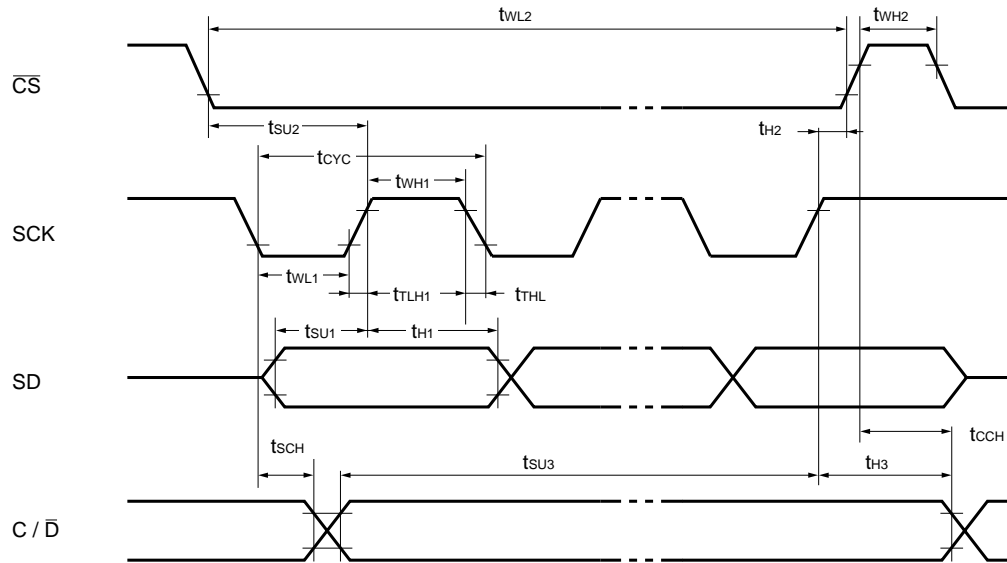
Fig. 2 Interface timing
