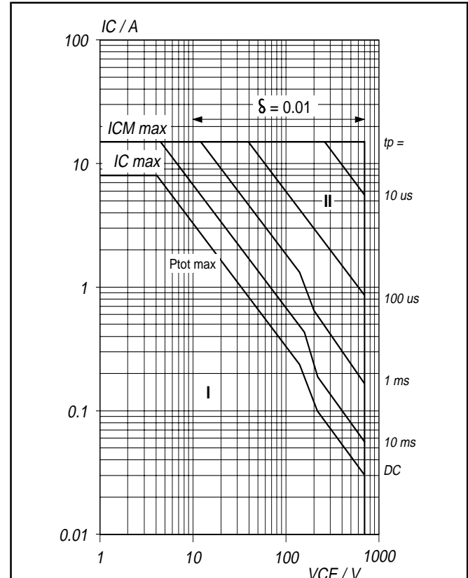
Fig.11. Forward bias safe operating area. T_{hs} = 25^\circ\text{C} I Region of permissible DC operation. II Extension for repetitive pulse operation.
