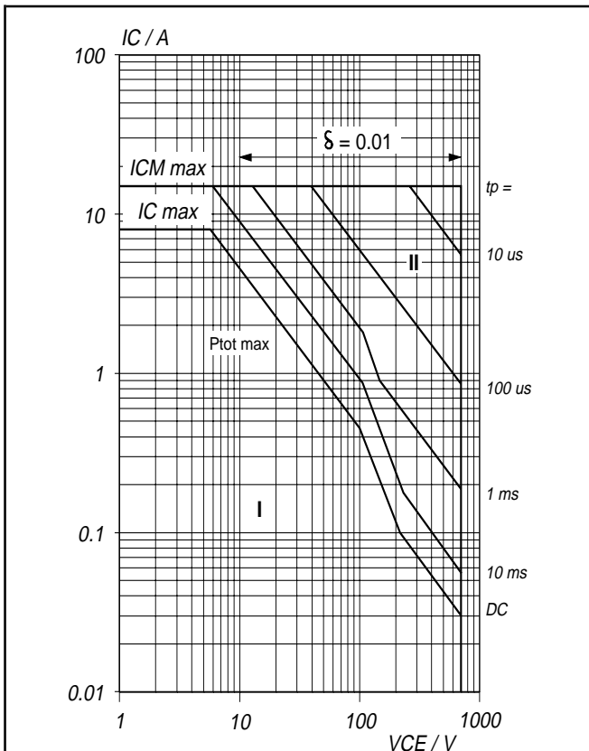
Fig.10. Forward bias safe operating area. T_{hs} = 25^\circ\text{C} I Region of permissible DC operation. II Extension for repetitive pulse operation.
