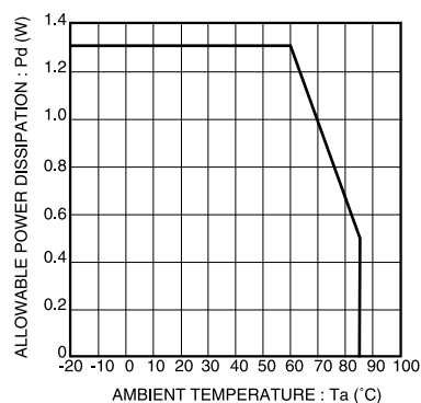
Fig.4 Derating curve when 2-outputs simultaneous operating
