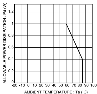
Fig.3 Derating curve of 1-output
