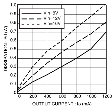
Fig.7 Circuit dissipation at Vo=5.0V
