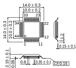
QFP44
