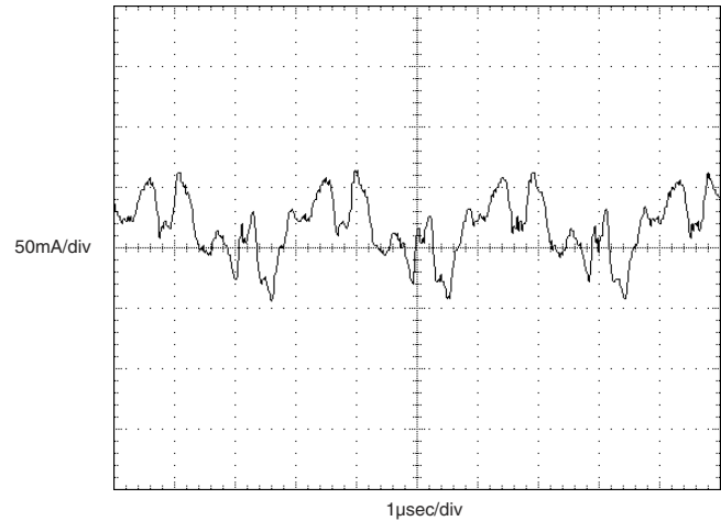
(VIN = 48V, 5V @ 15A, 3.3V @ 0A, external 22 \mu F low-ESR input capacitor.)
