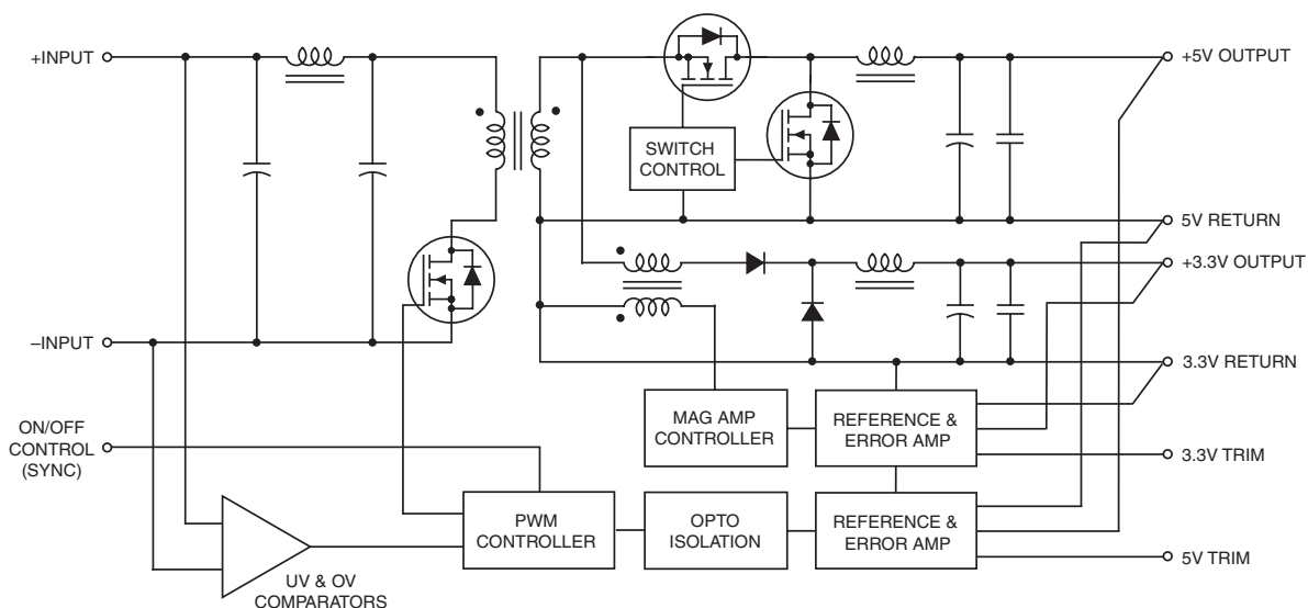
Figure 1. Simplified Schematic
