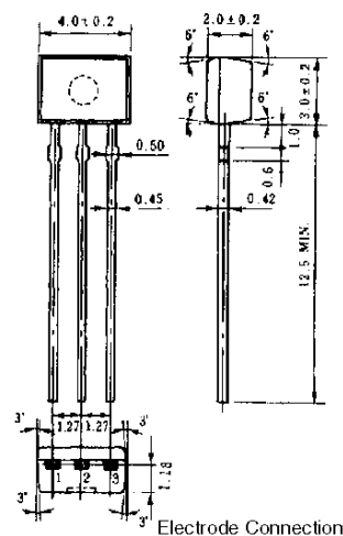
Electrode Connection 1. Emitter 2. Collector 3. Base
